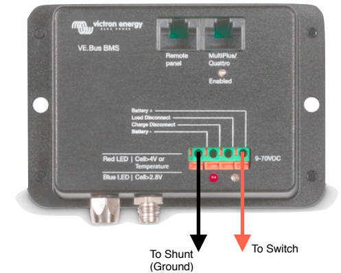
VE.Bus BMS Connection Points
